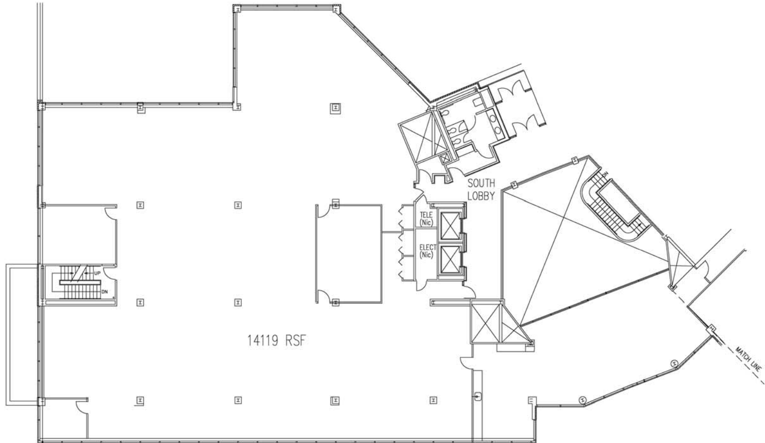
A PARTIAL FLOOR PLAN – SEGMENT A– 14119 RSF THIRD FLOOR SOUTH SCALE: 1/8" = 1'-0"
